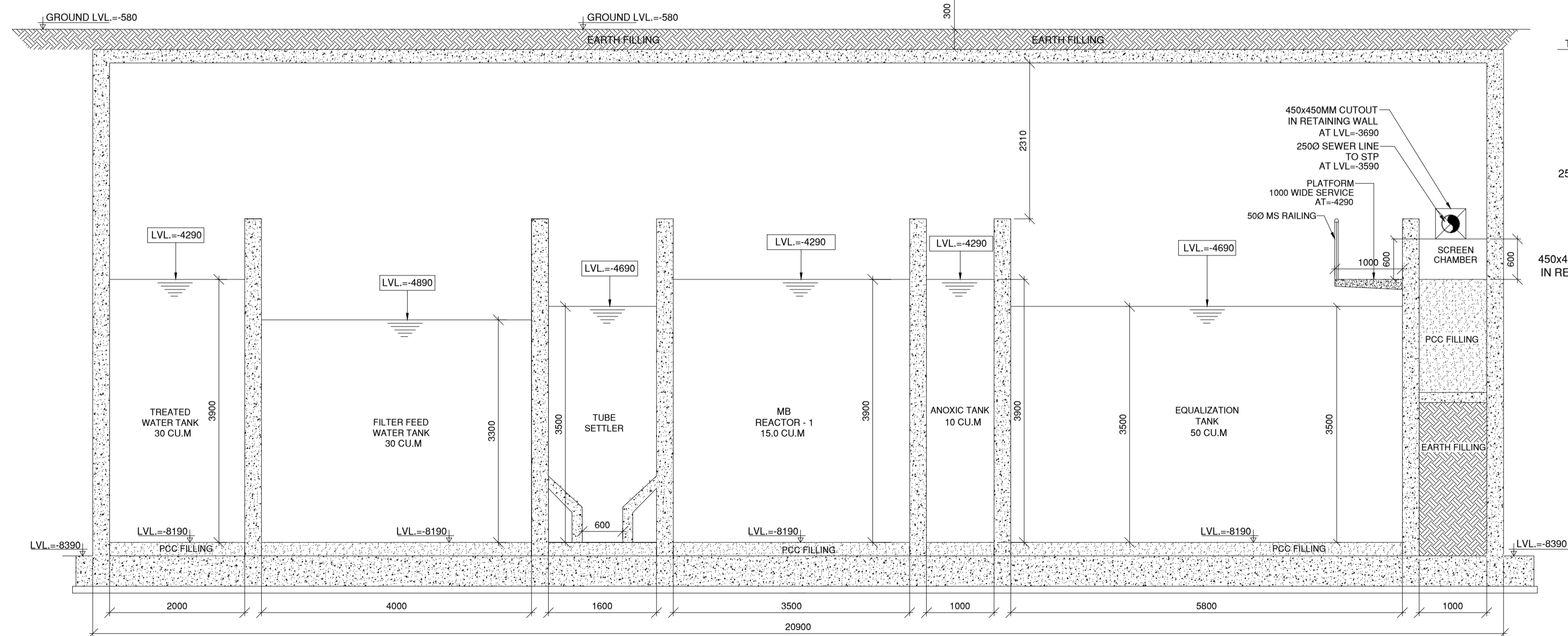
SECTION-AA
